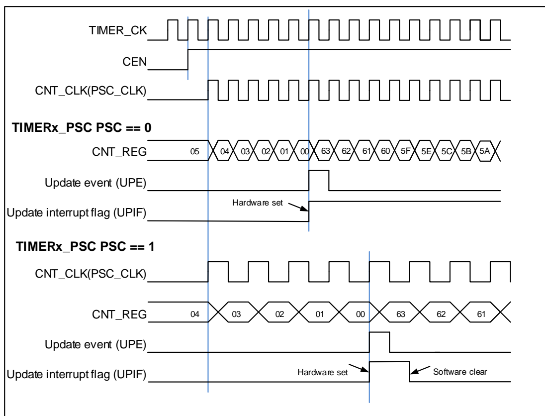
Figure 15-39. Timing chart of down counting mode, PSC=0/1
