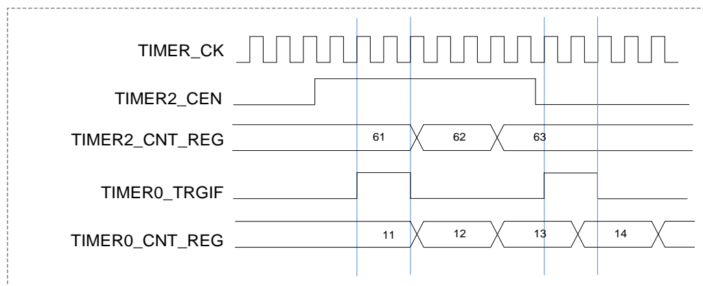
Figure 15-29. Triggering TIMER0 with enable signal of TIMER2
