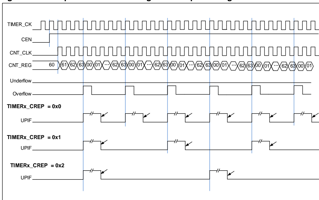
Figure 15-10. Repetition counter timing chart of up counting mode
