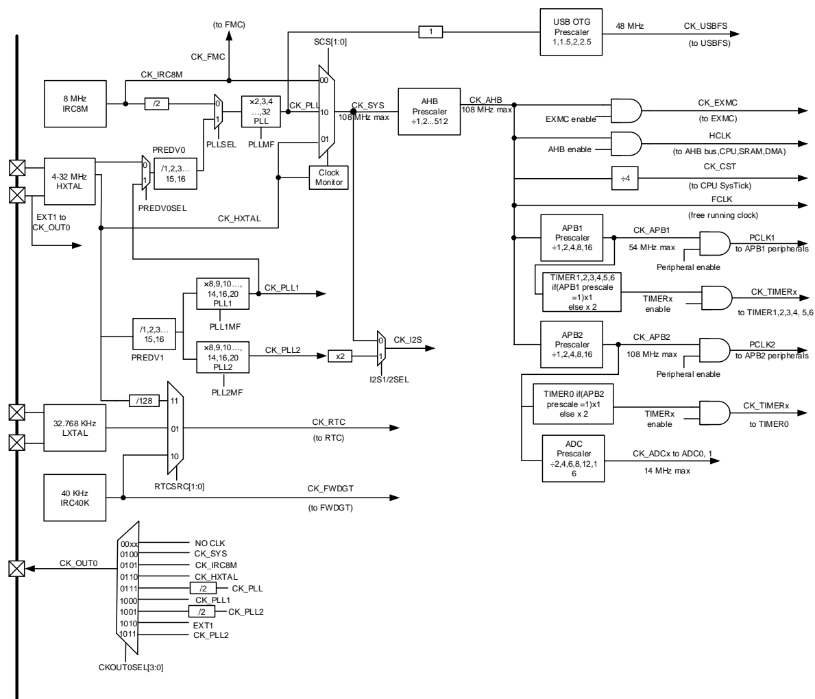
Figure 5-2. Clock tree
