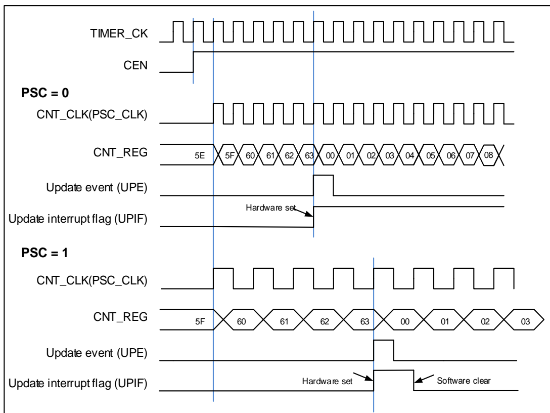
Figure 15-37. Timing chart of up counting mode, PSC=0/1
