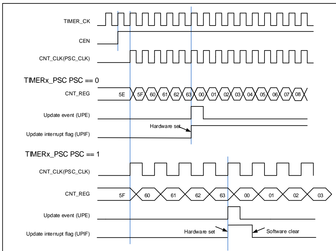
Figure 15-55. Timing chart of up counting mode, PSC=0/1
