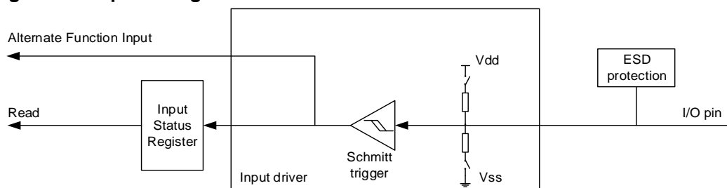
Figure 7.2. Input configuration
