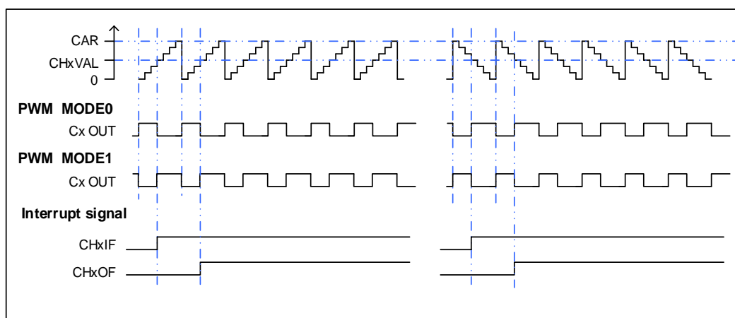
Figure 15-44. EAPWM timechart
