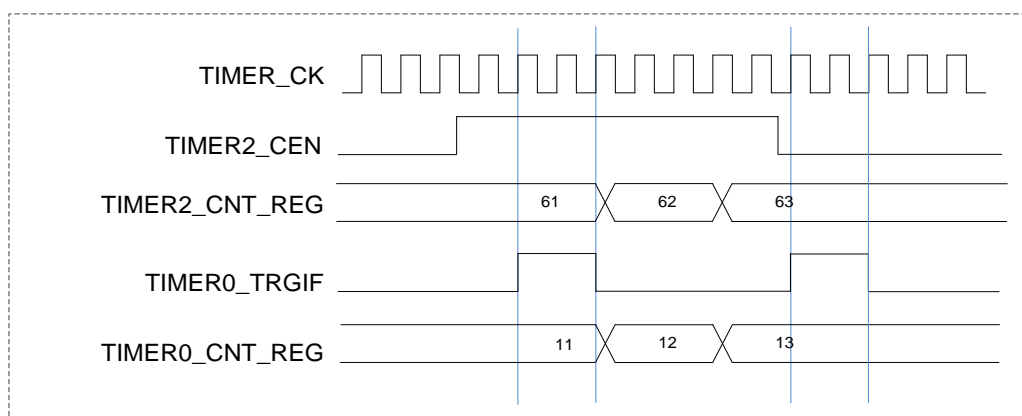
Figure 15-32. Pause TIMER0 with O0CPREF signal of Timer2
