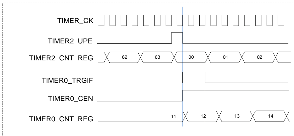
Figure 15-30. Triggering TIMER0 with update signal of TIMER2
