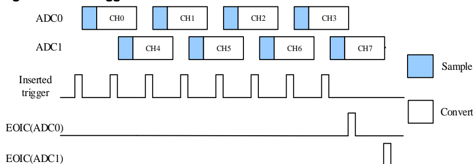
Figure 11-19. Trigger rotation: inserted channels in discontinuous mode
