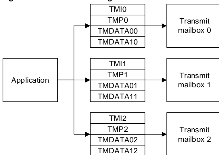
Figure 20-2. Transmission register
