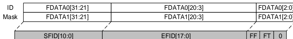
Figure 20-7. 32-bit mask mode filter
