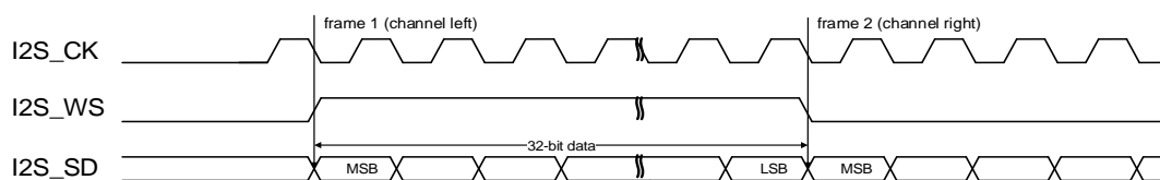
Figure 18-22. MSB justified standard timing diagram (DTLEN=10, CHLEN=1, CKPL=0)
