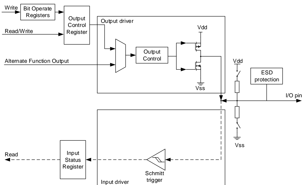
Figure 7.3. Output configuration
