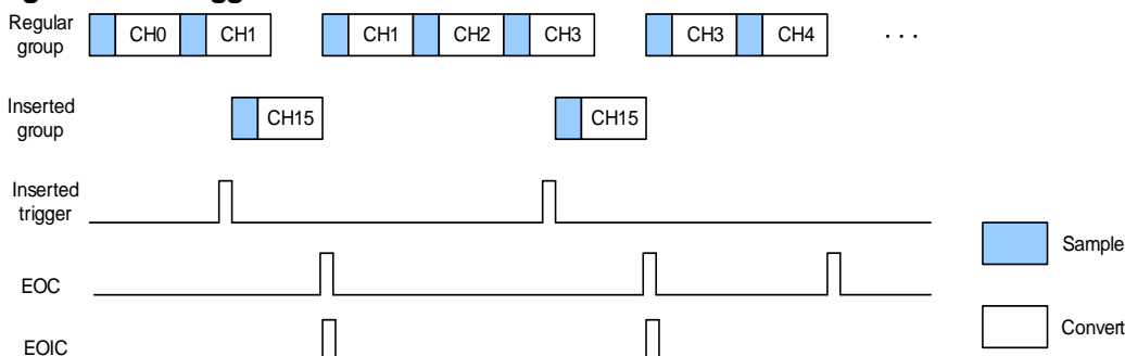
Figure 11-8. Triggered insertion
