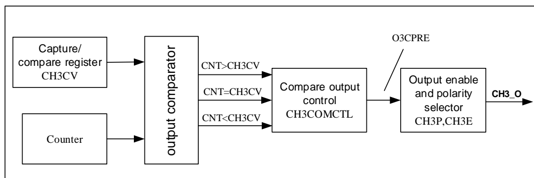
Figure 15-14. Output compare logic (CH3_O)
