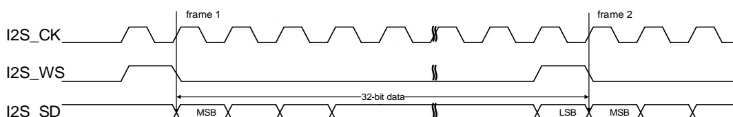
Figure 18-34. PCM standard short frame synchronization mode timing diagram (DTLEN=10, CHLEN=1, CKPL=0)
