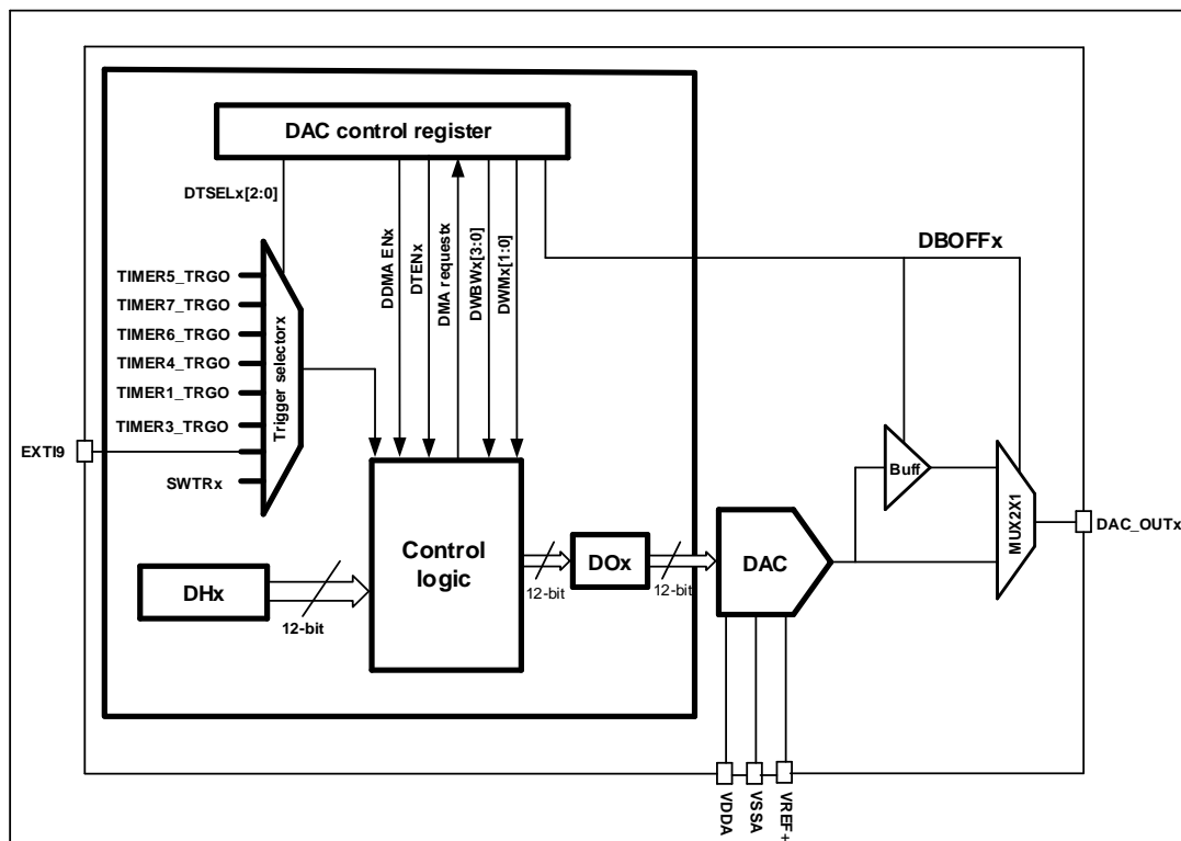
Figure 12-1. DAC block diagram
