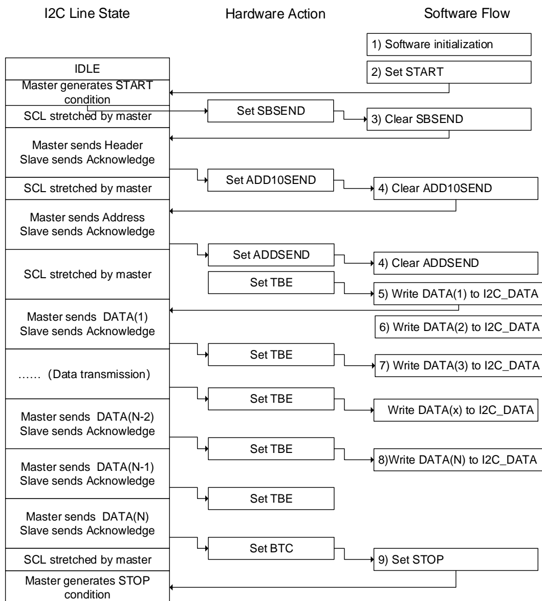
Figure 17-11. Programming model for master transmitting(10-bit address mode)
