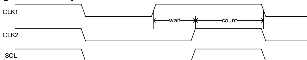
Figure 17-4. Clock synchronization
