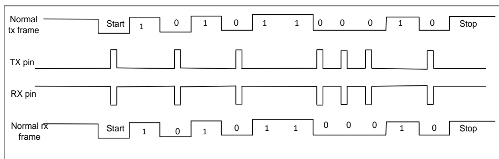
Figure 16-14. IrDA data modulation
