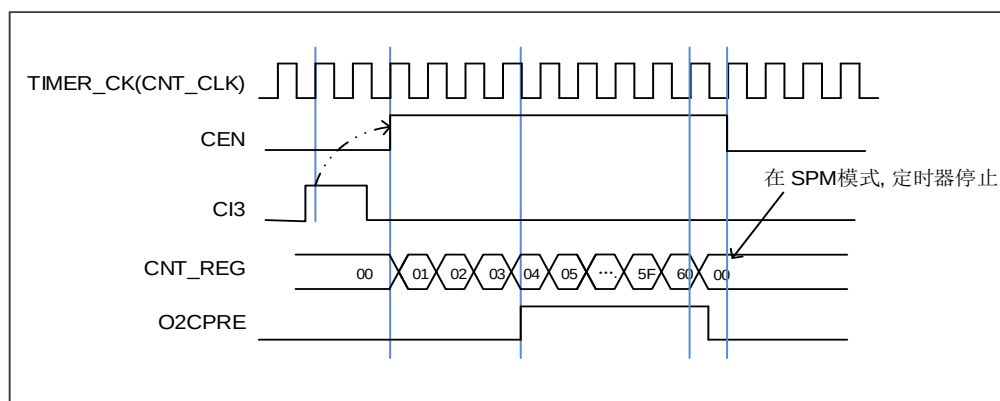
图 15-27. 单脉冲模式, TIMERx_CHxCV = 0x04 , TIMERx_CAR=0x60
