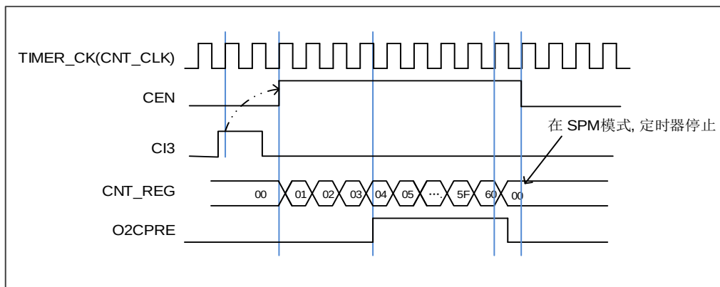
图 15-51. 单脉冲模式, TIMERx_CHxCV = 0x04 , TIMERx_CAR=0x60
